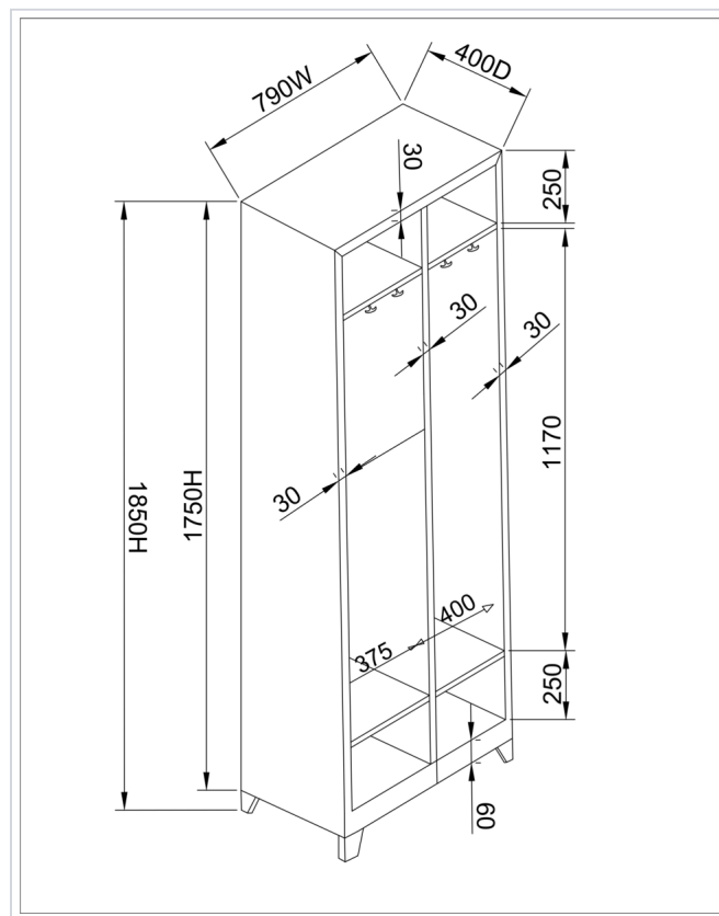
Internal dimensions
