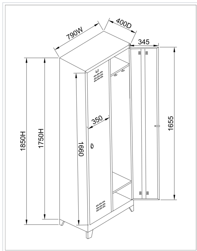
Exterior view with interior layout
