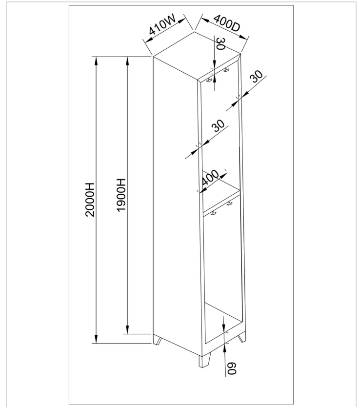
Internal dimensions
