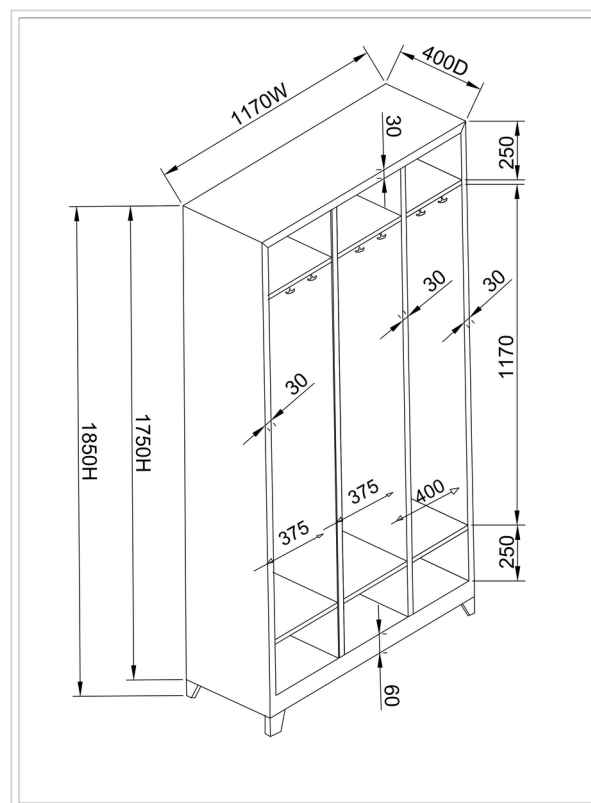
Internal dimensions
