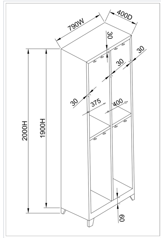
Internal dimensions
