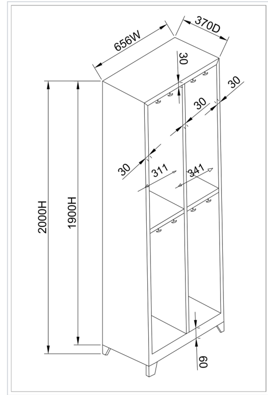
Internal dimensions
