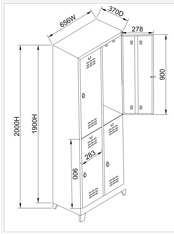
Exterior view
