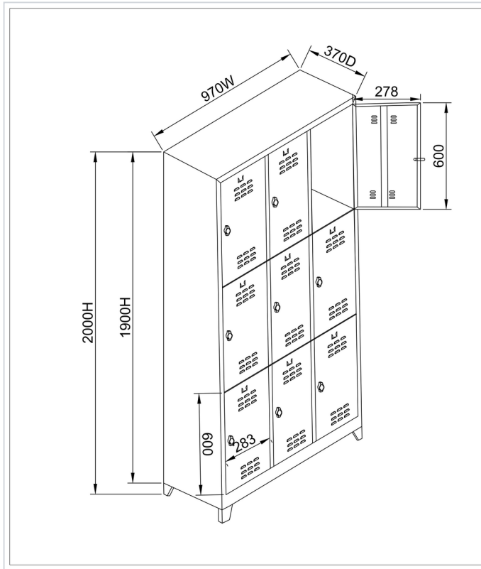
Exterior view
