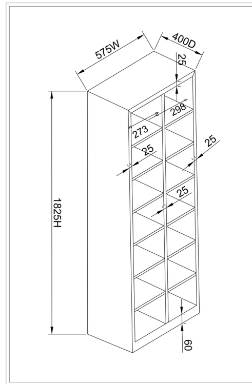
Internal dimensions
