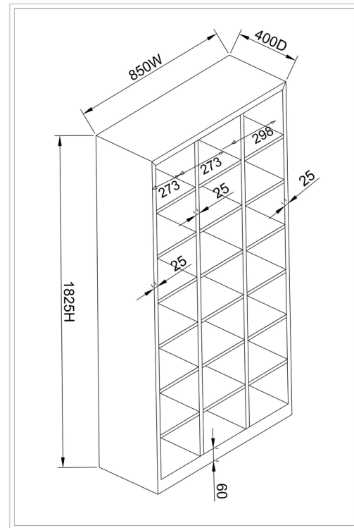
Internal dimensions
