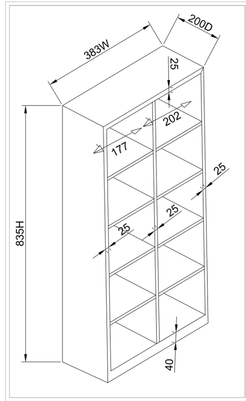
Internal dimensions
