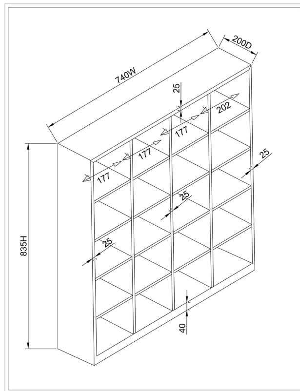
Internal dimensions
