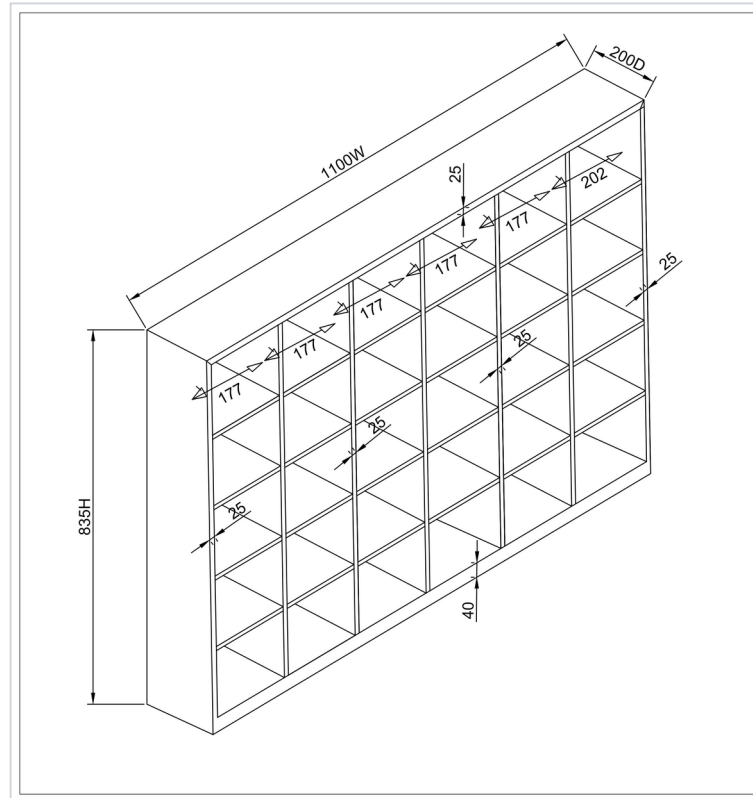
Internal dimensions
