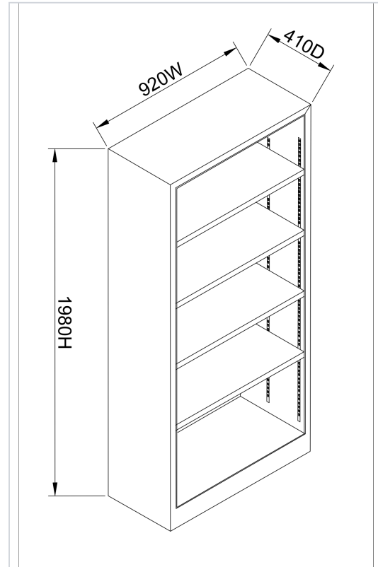
Interior, doors removed (1980 mm shown)
