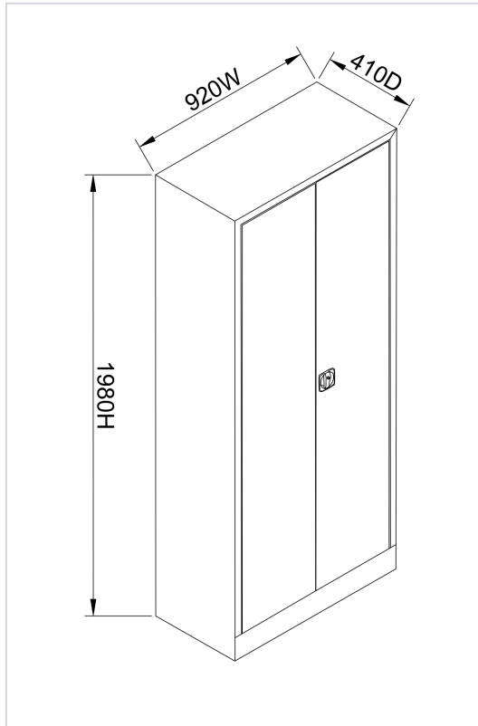
Exterior, doors closed (1980 mm shown)
