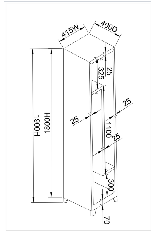
Internal dimensions
