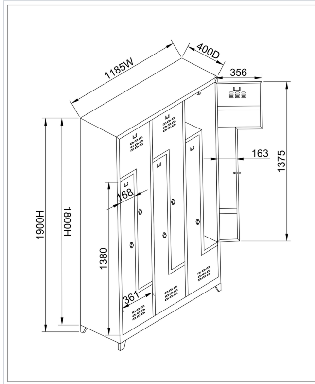
Exterior view
