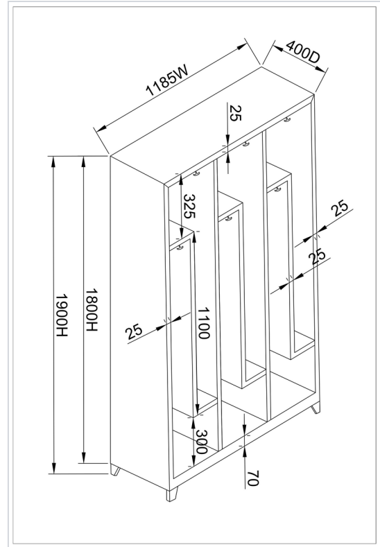
Internal dimensions
